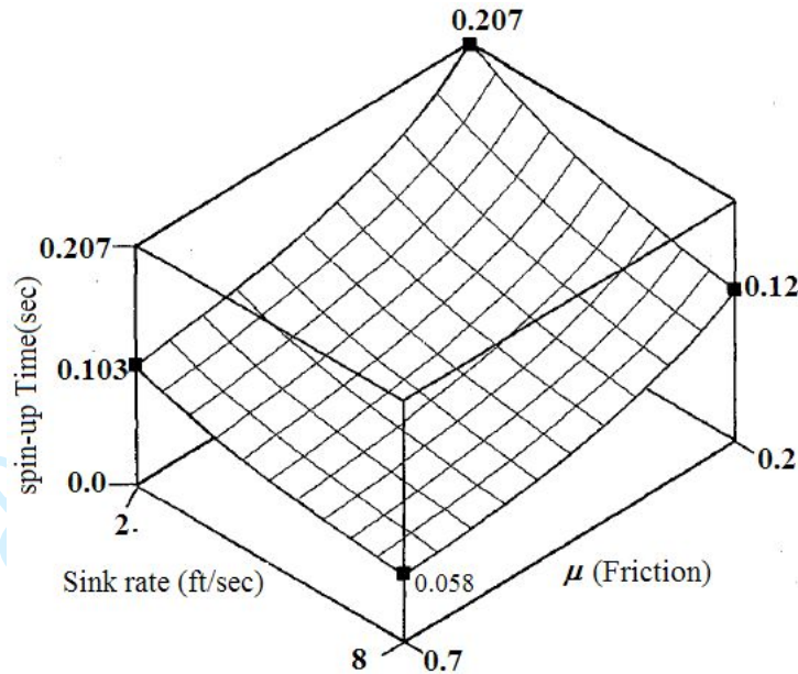
Fig. 4 Parametric effects of sink rate and friction coefficient on the skidding distance or spin-up time
