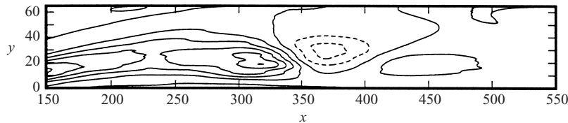
FIGURE 11. SEP: Contours of shear production ( -\langle u'v' \rangle \partial u / \partial y ) of turbulent kinetic energy. Positive values shown as solid lines, negative as dashed. Values from -3.5 to 8.5 .
