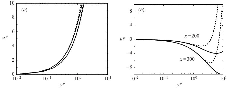
FIGURE 16. Velocity profiles in pressure gradient scaling. (a) APG1: —, DNS; ----, \frac{1}{2}(y^p)^2 + (u_\tau/u_p)^2 y^p . (b) SEP: —, DNS; ----, \frac{1}{2}(y^p)^2 - (u_\tau/u_p)^2 y^p .
