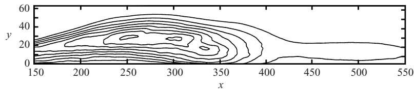
FIGURE 10. SEP: Contours of turbulent kinetic energy. Values from 0.005 to 0.025.
